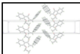
Fig. 2. The crystal packing of the title compound viewed along the b axis, showing chains running along the a axis. C—H...O weak interactions are shown as dashed lines.
